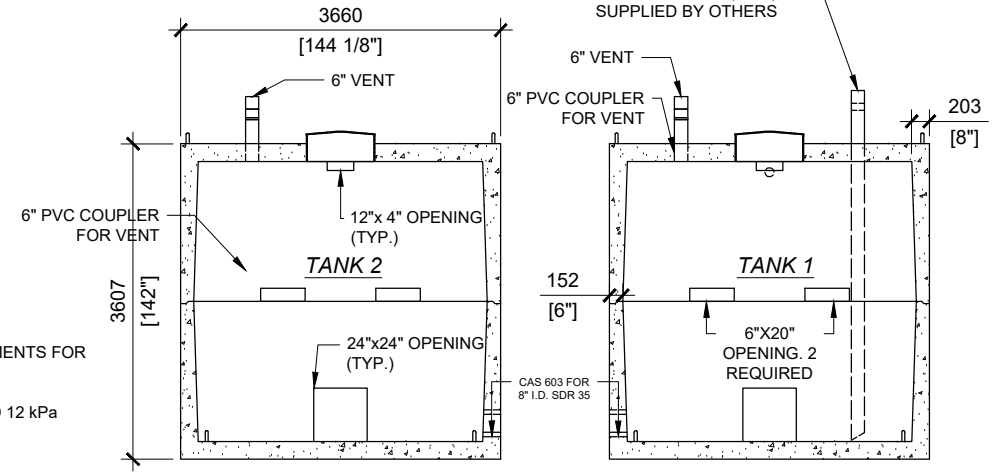
SECTION B SCALE 1:90
