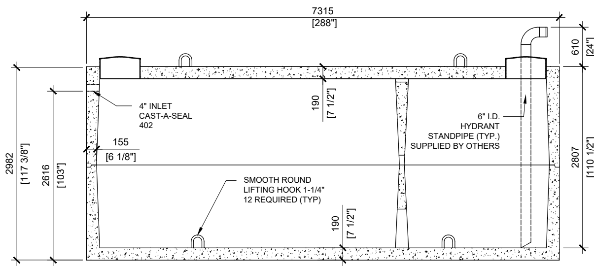
SECTION A SCALE 1:60
