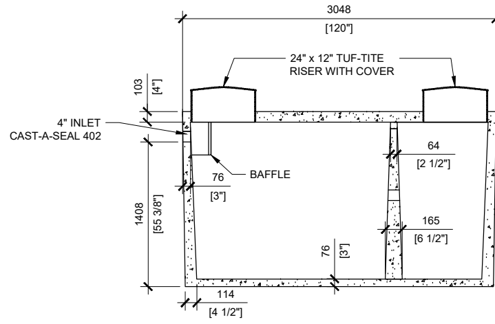
SECTION A SCALE 1:50
