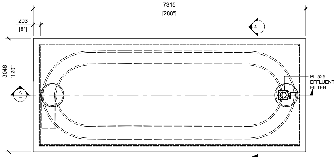
TOP VIEW SCALE 1:60
