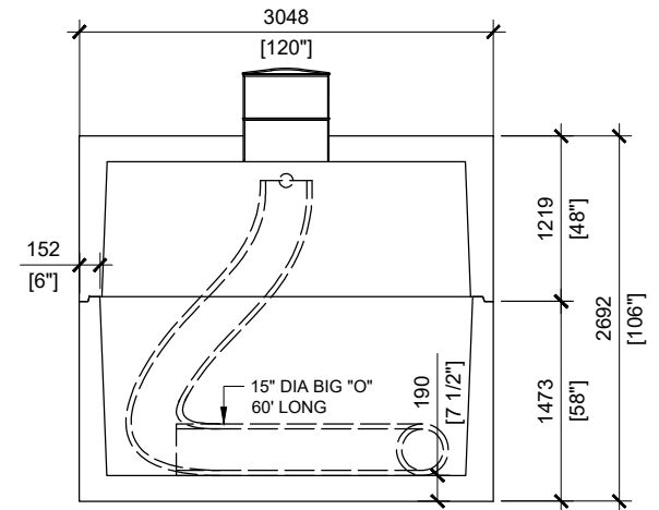
SECTION B SCALE 1:60
