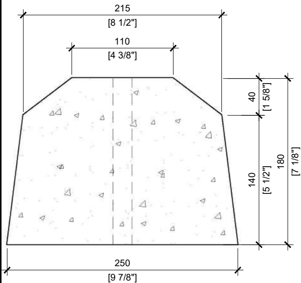
SIDE VIEW SCALE 1/4
