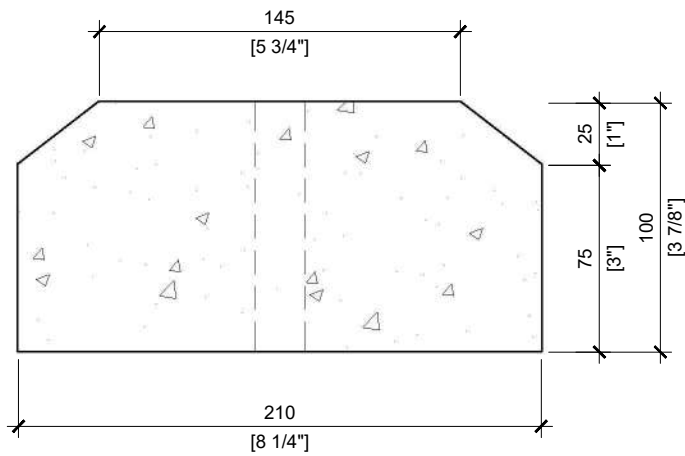
SECTION VIEW SCALE 1/3
