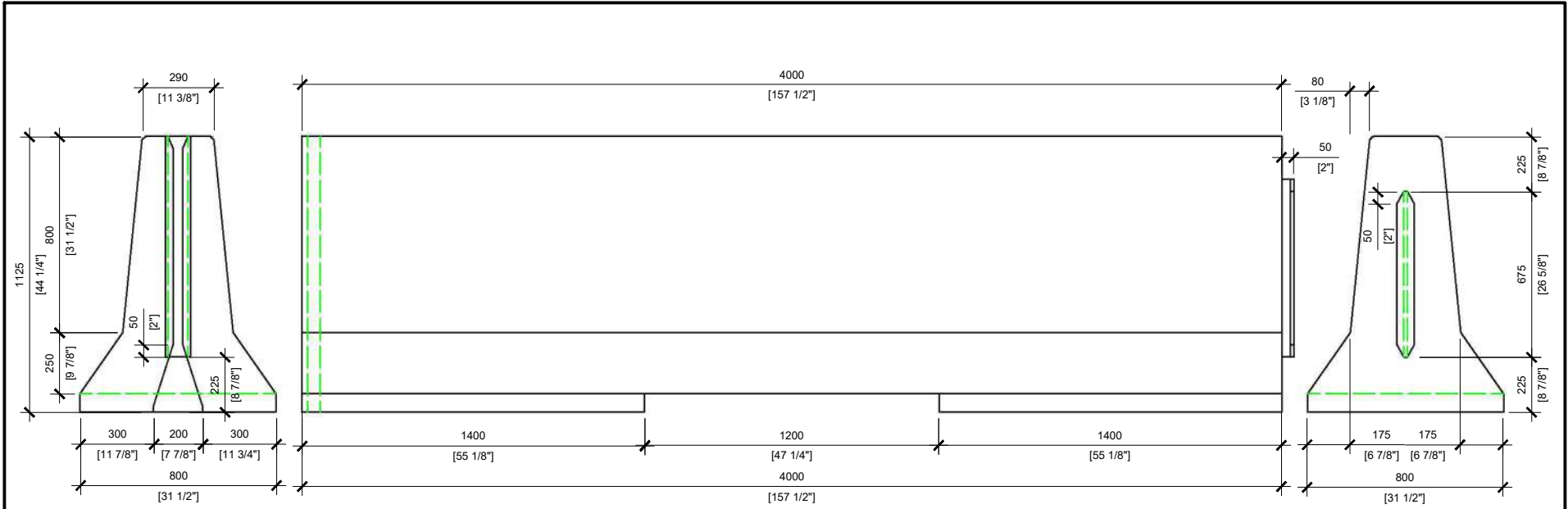
FEMALE END VIEW SCALE: 1:25
