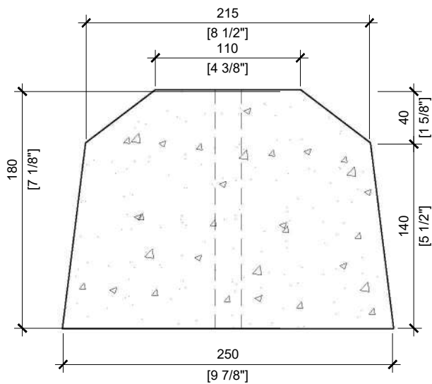
SIDE VIEW SCALE 1/4
