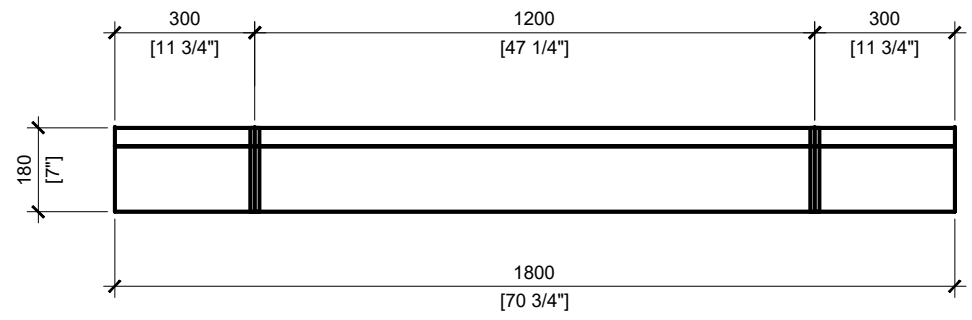
FRONT VIEW SCALE 1/16
