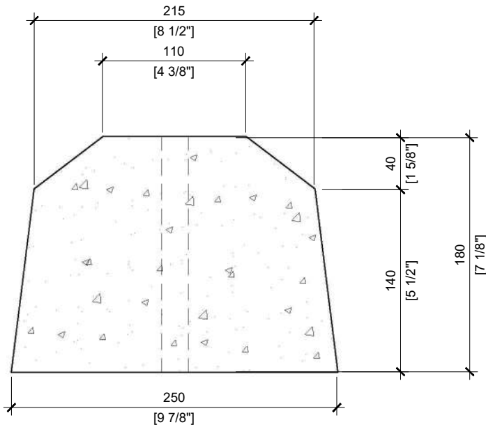
SIDE VIEW SCALE 1/4
